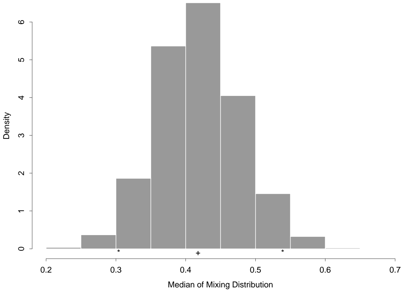
Figure 5: Histogram for median mixing proportions – model B. This histogram show the distribution of MCMC realizations for the median of the mixing proportion distribution, \mu_x . The median of this distribution is approximately 0.42, and a 95% credible interval is (0.30, 0.54).
