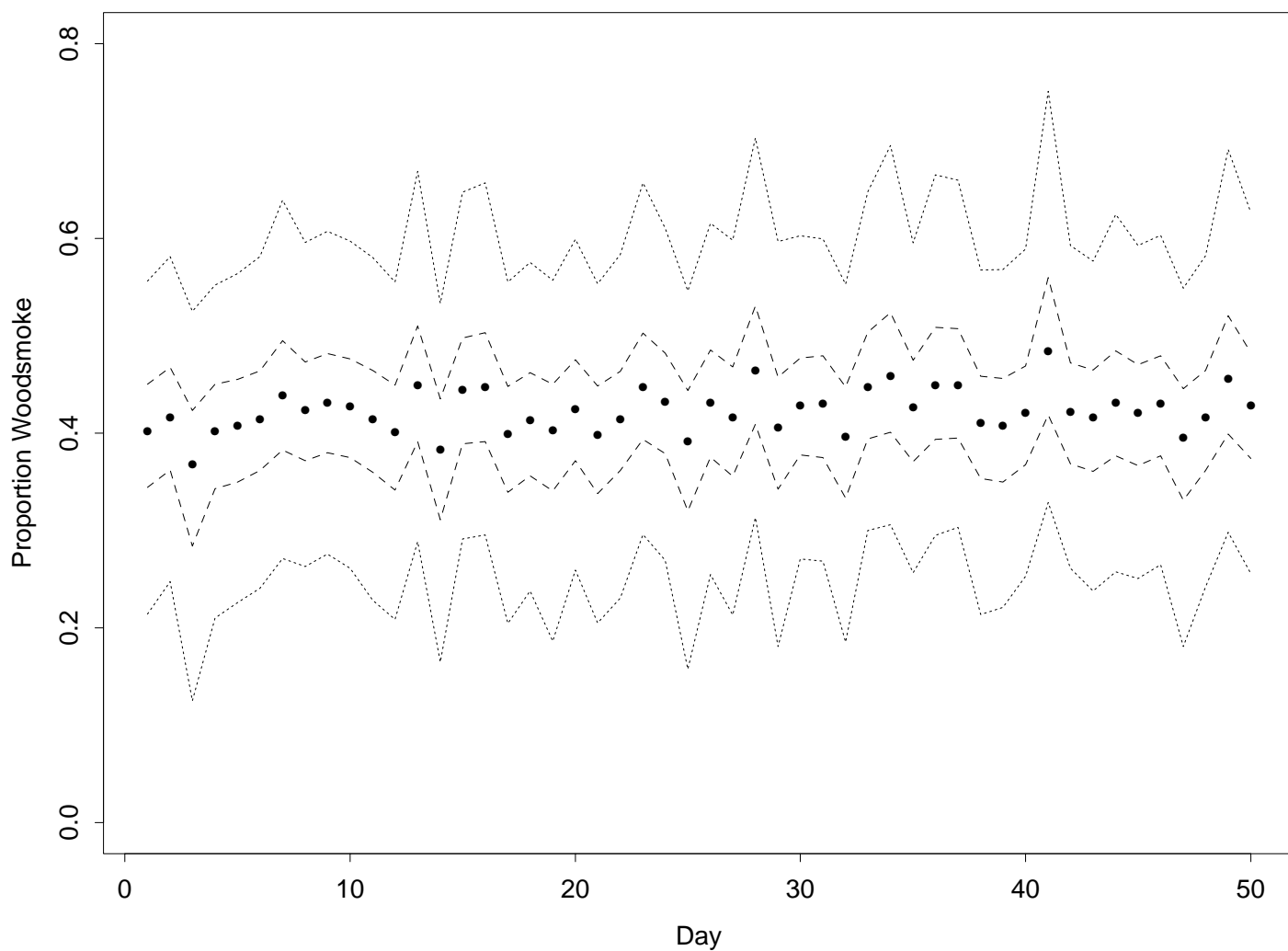
Figure 4: Point estimates and credible intervals for daily wood-smoke proportion – model B. Points indicate median proportion attributable to wood-smoke for each daily observation. 50% and 95% credible intervals are indicated by dashed and dotted lines, respectively.
