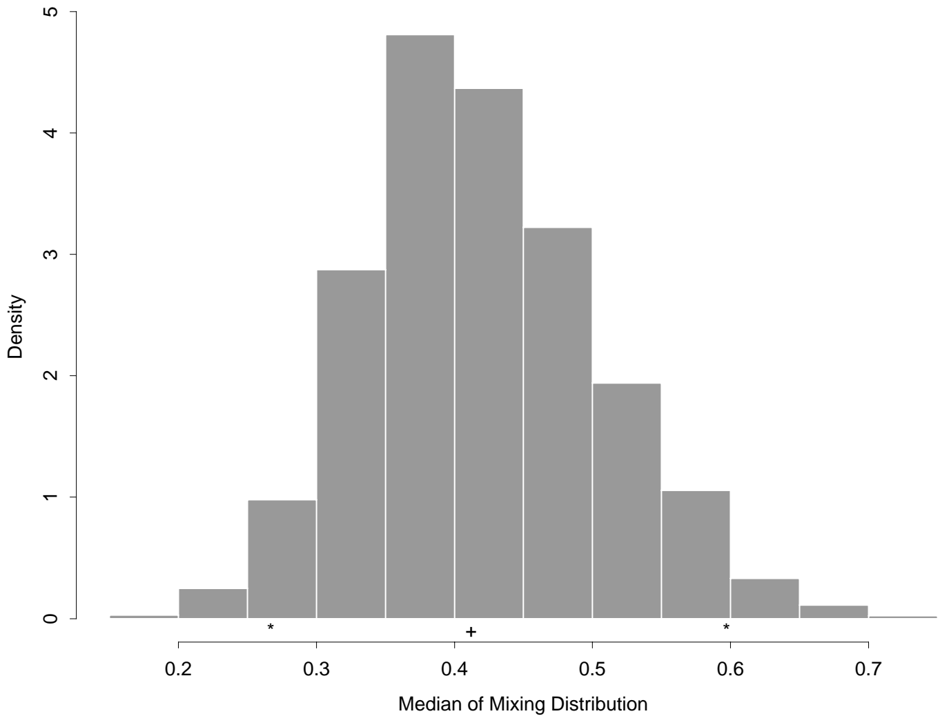
Figure 2: Histogram for median mixing proportions. This histogram show the distribution of MCMC realizations for the median of the mixing proportion distribution, \mu_\alpha . The median of this distribution is approximately 0.41, and a 95% credible interval is (0.27, 0.60).
