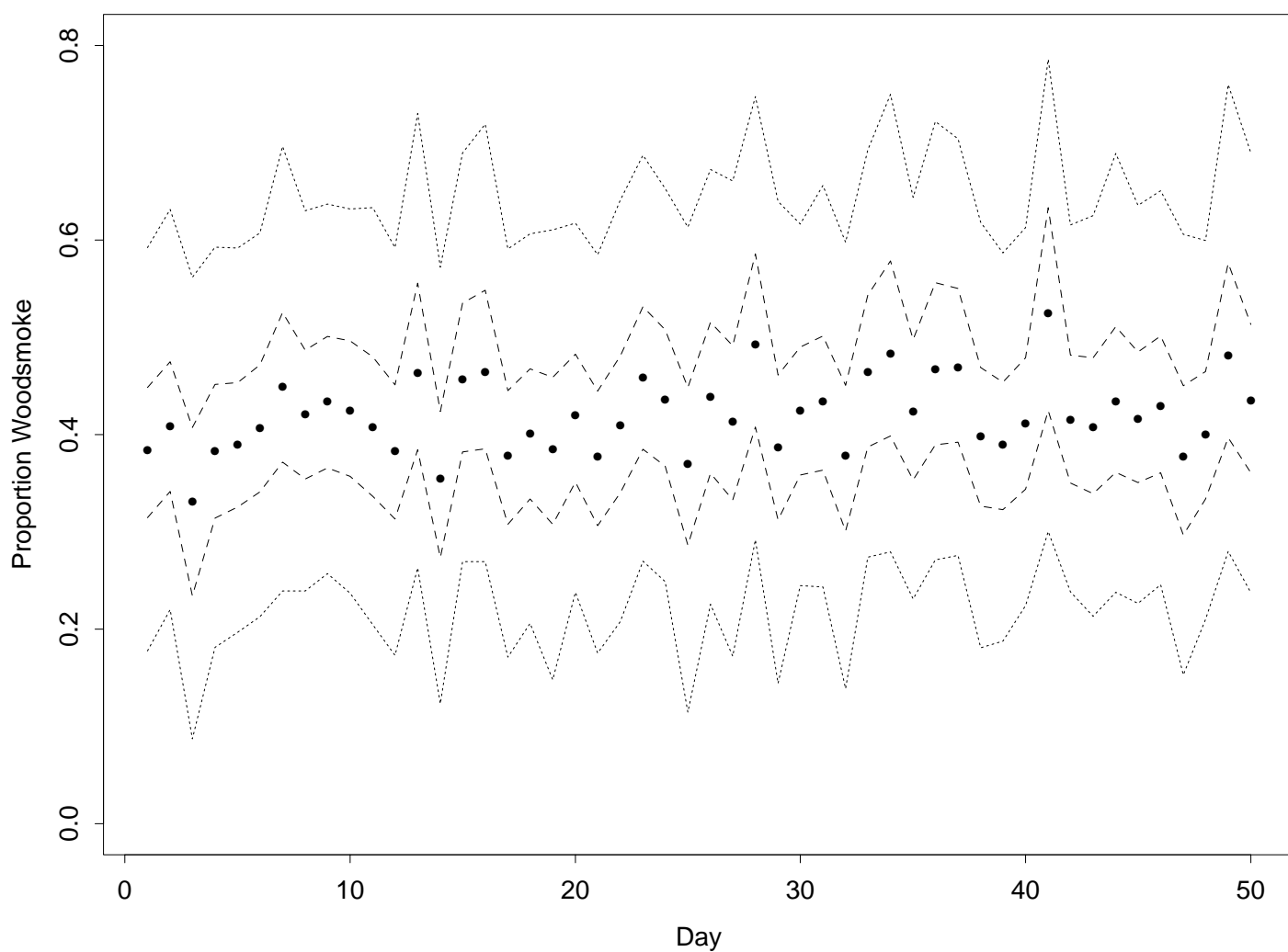
Figure 1: Point estimates and credible intervals for daily wood-smoke proportion. Points indicate median proportion attributable to wood-smoke for each daily observation. 50% and 95% credible intervals are indicated by dashed and dotted lines, respectively.
