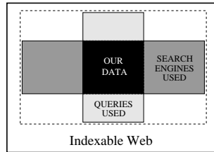
Fig. 2. The two populations of Web pages which define the observed data
