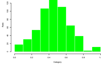
Fig. 1. Proportion of Petersen estimates smaller than n_k
