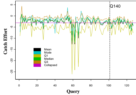
Fig. 6. Catchability effect of Alta Vista across the queries selected in the sample. The vertical axis represents the number value of \beta_1 in model (7) and the curves connect the quantiles of the 128 sample queries displayed along the horizontal axis in an arbitrary order
