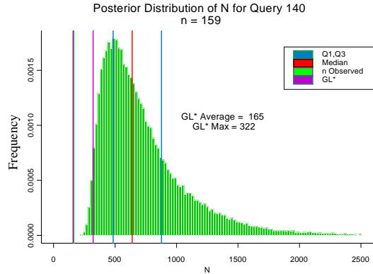
Fig. 3. Posterior distribution of the projected number of Web pages N_k for query Q_{140}
