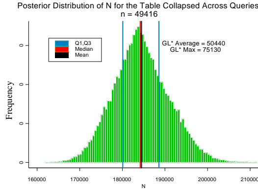
Fig. 5. Posterior distribution of \mathcal{N} for the seven-way table \mathcal{S} aggregated across queries
