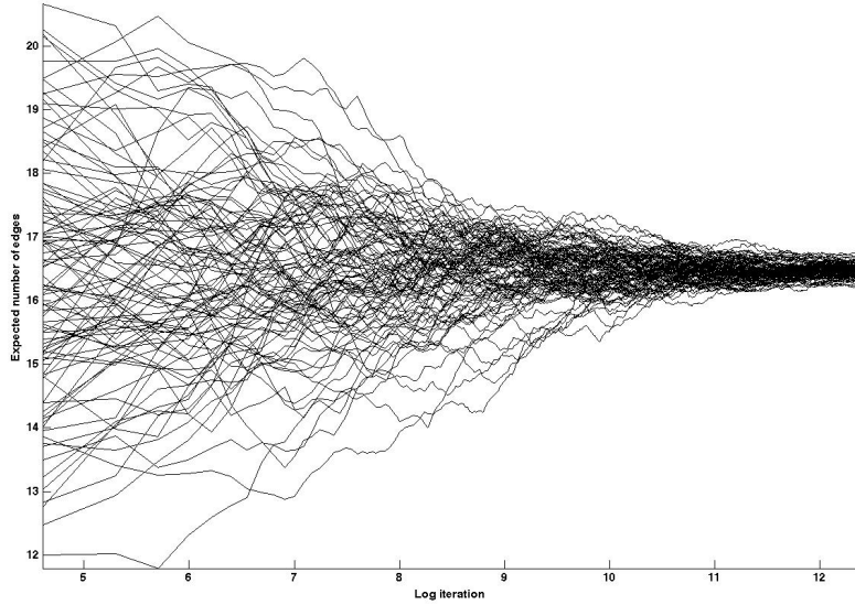
FIG 5.1. Estimates of the posterior expected number of edges in the CGGMs for the Rochdale data.
