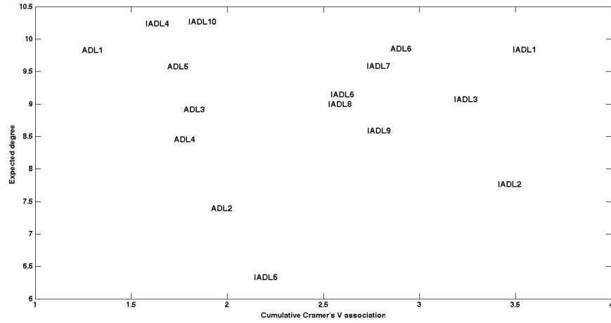
Fig 5.3. Cumulative Cramer's V associations (x-axis) and posterior expected degrees (y-axis) of the 16 disability measures from the NLTCs functional disability data.
