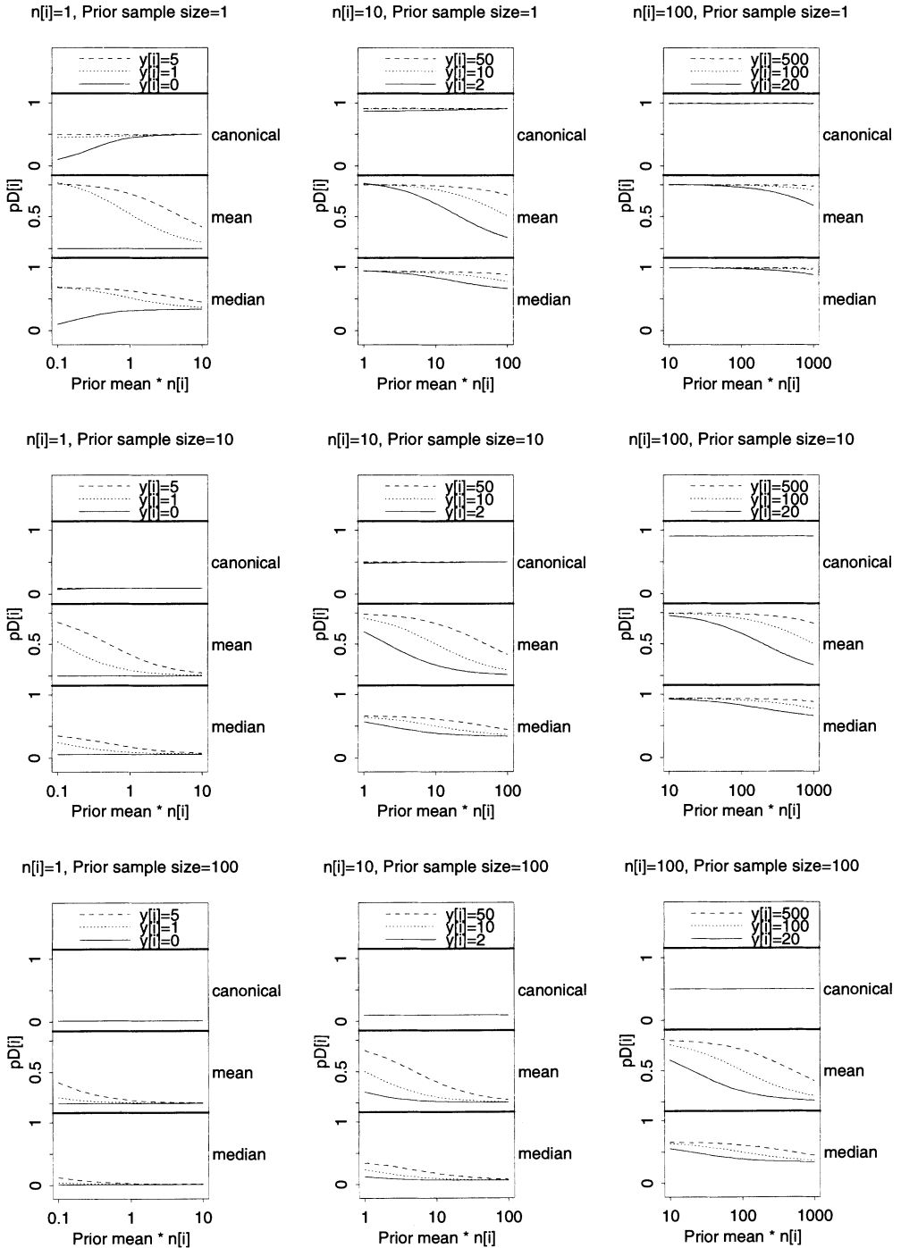
Fig. 2. Poisson likelihood—contribution of the i th group to the effective number of parameters under various parameterizations (canonical p_{D_i}^0 , mean p_{D_i}^\mu , and median p_{D_i}^{\text{med}} ) as a function of the data (sample size n_i and observed total y_i ) and prior (mean n_i a/b and 'sample size' b )
