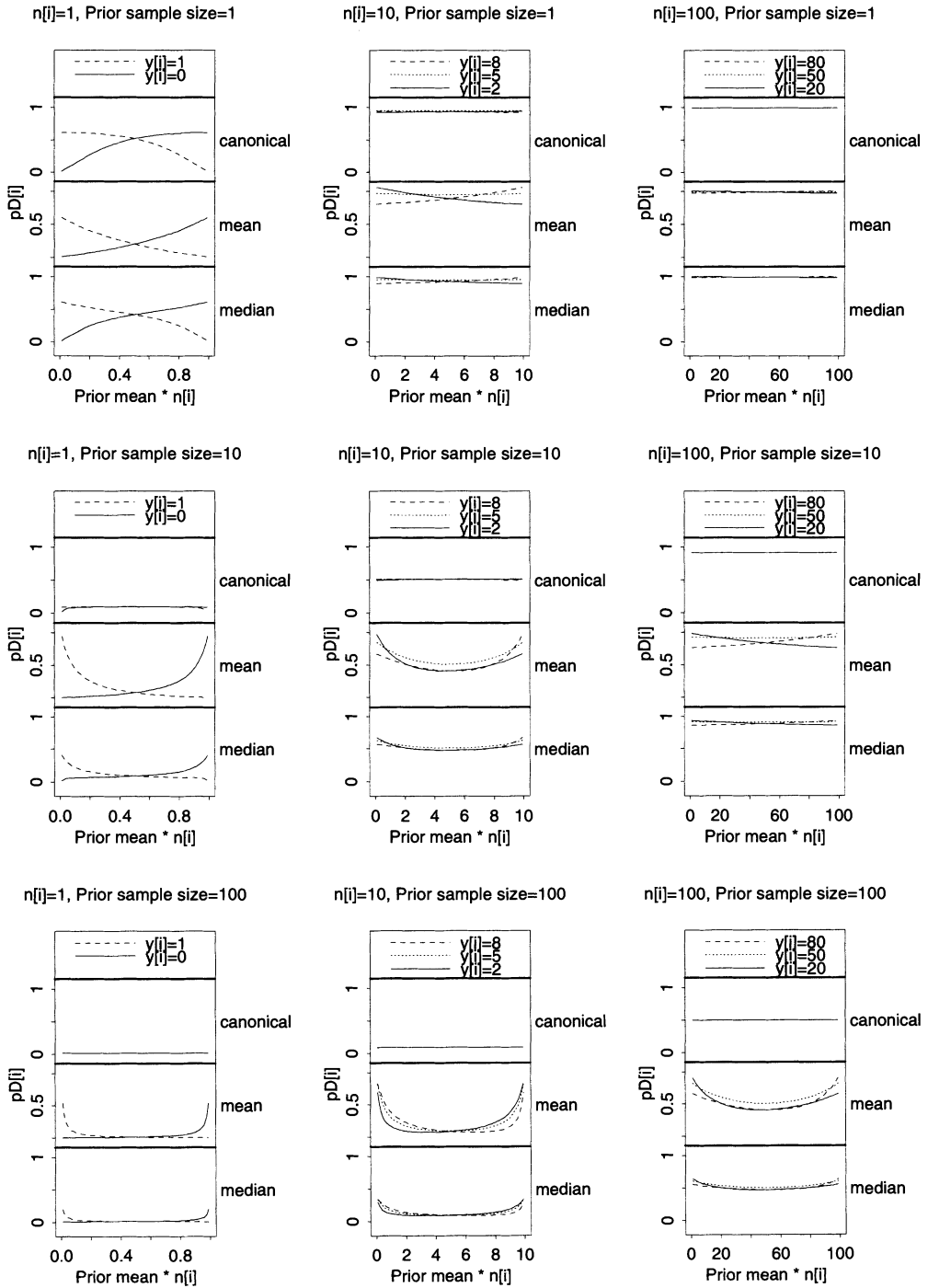
Fig. 1. Binomial likelihood—contribution of the i th group to the effective number of parameters under various parameterizations (canonical p_{D_i}^{\text{can}} , mean p_{D_i}^{\text{m}} and median p_{D_i}^{\text{med}} ) as a function of the data (sample size n_i and observed proportion y_i/n_i ) and prior (effective prior sample size a+b and prior mean a/(a+b) ): we are seeking agreement between alternative parameterizations with little dependence on data
