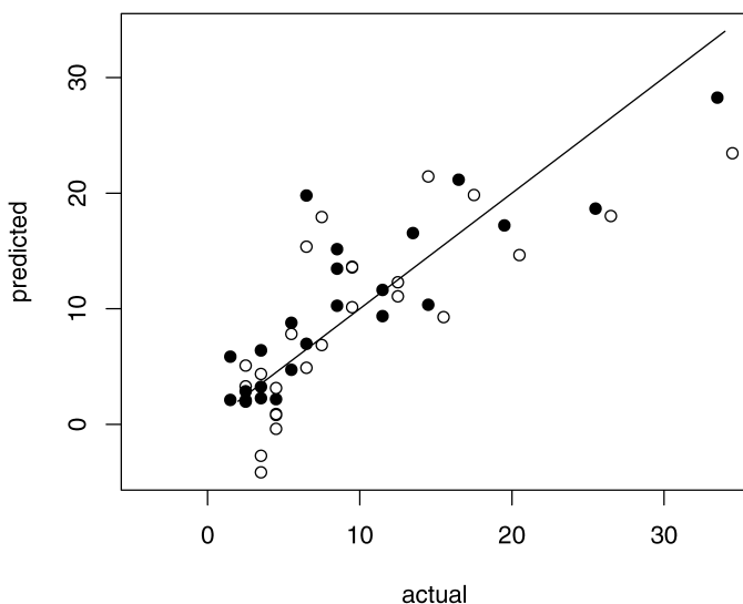
Figure 1. Scatterplot of Observed versus Predicted, Using the Prediction Dataset, for the Breiman–Friedman Model ( \circ ) and the Third Model of Table 6 ( \bullet ).
