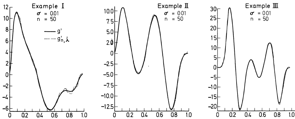
Fig. 5. The derivative g' and its estimate g'_{n,\hat{\lambda}}
