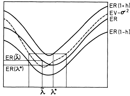
Fig. 1. Graphical suggestion of the proof of Theorem 4.2
