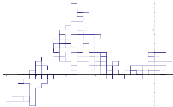
Figure 2: 2-dimensional simple random walk, X_i \sim \text{Uniform}\{(1, 0), (-1, 0), (0, 1), (0, -1)\} , n = 500
