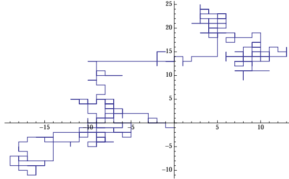
Figure 1: 2-dimensional simple random walk, X_i \sim \text{Uniform}\{(1, 0), (-1, 0), (0, 1), (0, -1)\} , n = 500
