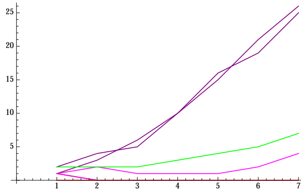
Figure 1: 8 sample paths, Galton-Watson branching process with Binomial(3, 1/2) offspring distribution
