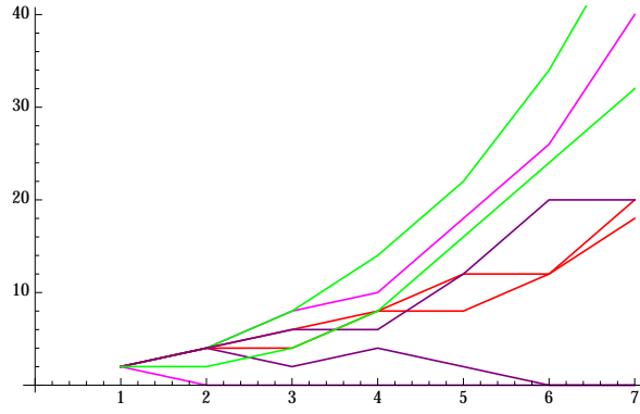
Figure 4: 8 sample paths, Galton-Watson branching process with Binary( a = 3/4 ) offspring distribution
