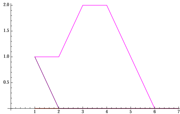
Figure 3: 8 sample paths, Galton-Watson branching process with Binomial(3, 1/4) offspring distribution
