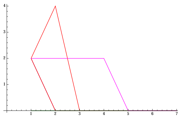
Figure 5: 8 sample paths, Galton-Watson branching process with Binary( a = 1/2 ) offspring distribution
