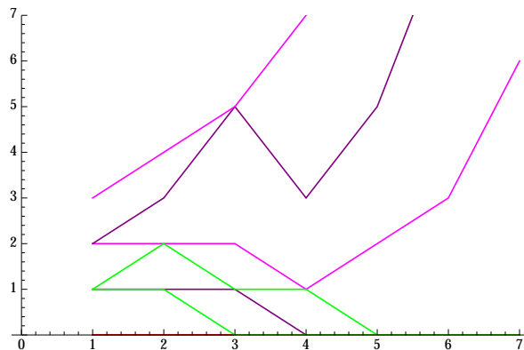
Figure 2: 8 sample paths, Galton-Watson branching process with Binomial(3, 1/3) offspring distribution
