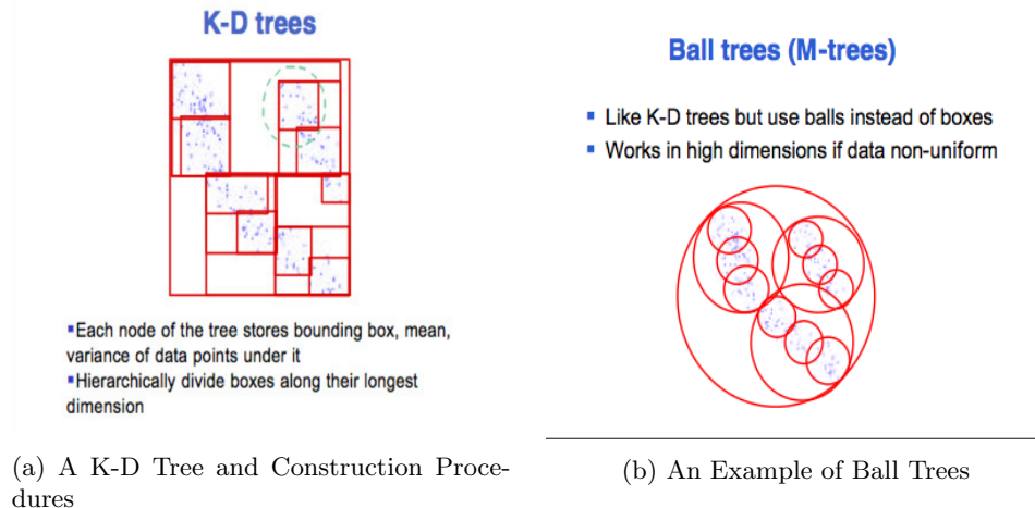
Figure 3: K-D Trees and Ball Trees
