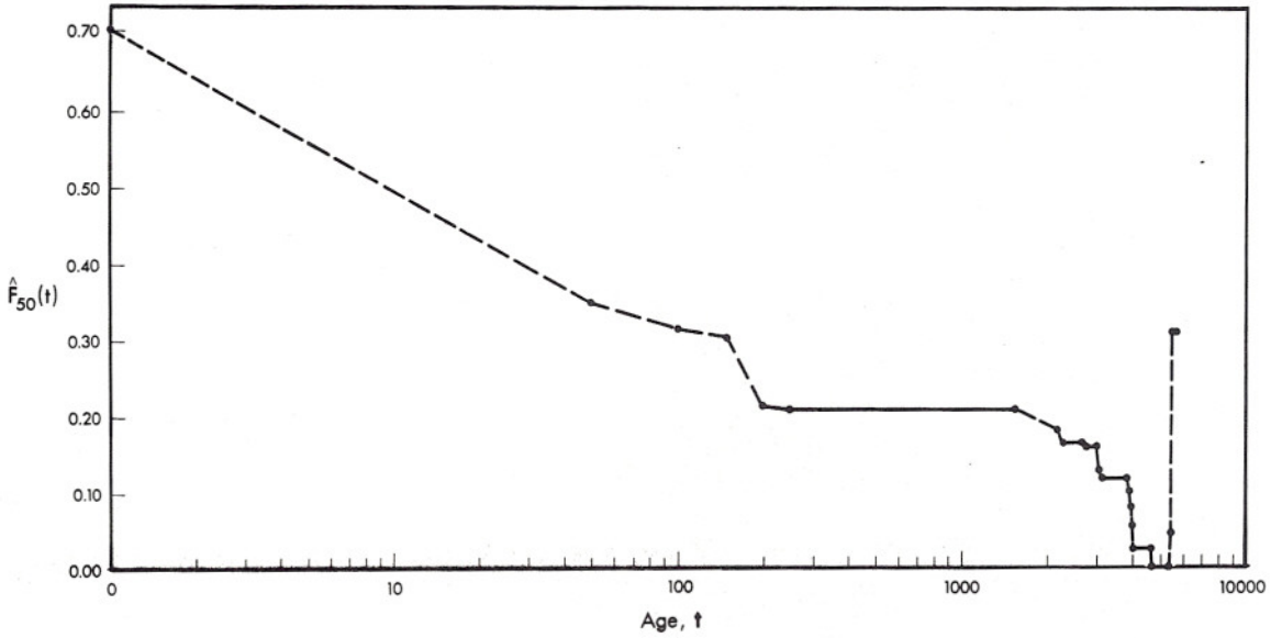
Fig. 5. MLE of \hat{F}_{50}(t) , of the conditional probability of failure in the next 50 hours given survival until age t
