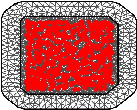
Constrained refined Delaunay triangulation
