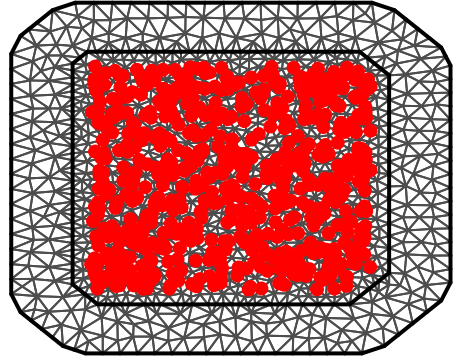
Constrained refined Delaunay triangulation
