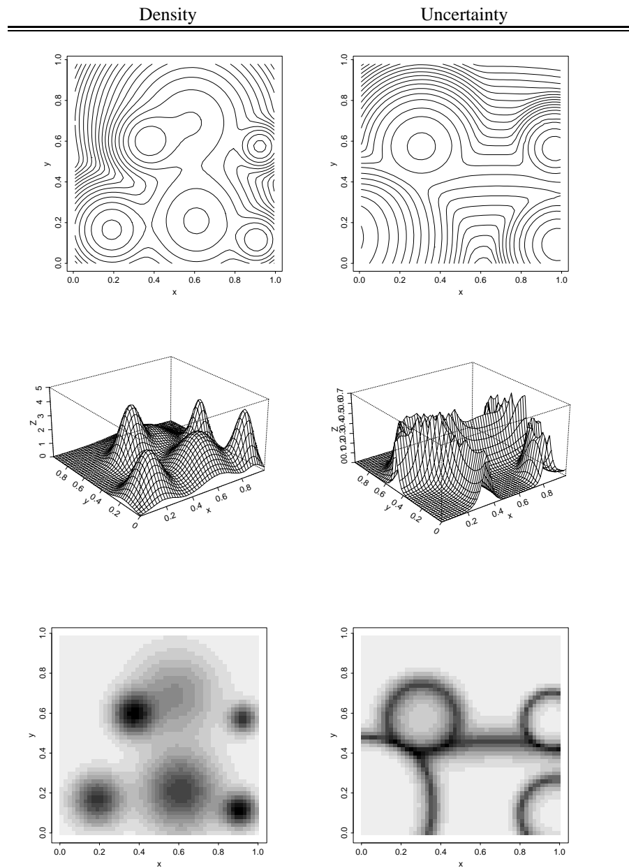
Figure 9. Density (left column) and uncertainty (right column) surfaces for the Lansing Woods maples. Contour, perspective, and image plots are displayed in the first, second, and third rows respectively. A logarithmic scale was used for the contour plots.
