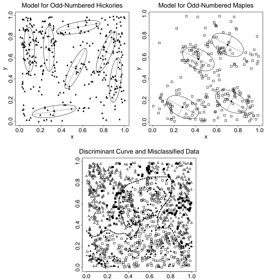
Figure 14. mclustDAttrain models and discriminant curve for the Lansing Woods data. Top Left: the hickory training [odd-numbered] class with its 7-group EEV model. Top Right: the maple training [odd-numbered] class with its 4-group EEE model. Bottom: discriminant curve with training and test errors (filled symbols).
