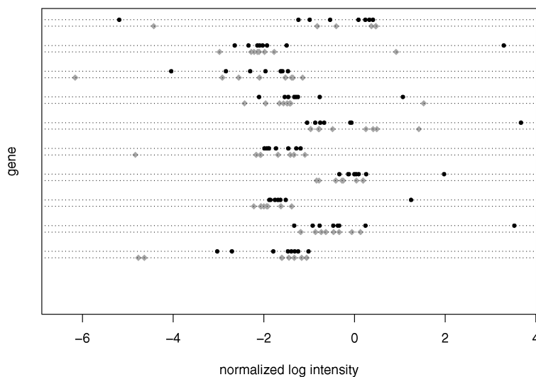
Figure 2. Dot Plots of 10 Genes From the Like-Like Data ( \bullet sample 1; \diamond sample 2). Even though the data were normalized, some replicate outliers are present in each sample.
