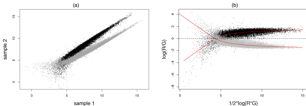
Figure 1. Effect of the Dye Swap on the Like-Like Data ( \bullet R = \text{sample 1} , G = \text{sample 2} ; \circ R = \text{sample 2} , G = \text{sample 1} ; — loess fit). (a) \log(\text{sample 1}) versus \log(\text{sample 2}) . This shows that the dye effect is approximately additive on the log scale. (b) Overall intensity versus log ratio. This shows that the nonlinear effects approximately cancel one another out in a balanced dye-swap experiment. The overall intensity is half the sum of the log intensities in the two channels, and all logarithms are to base 2.
