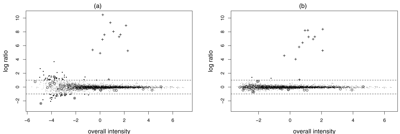
Figure 5. Log Ratio Estimates as a Function of the Overall Intensity (i.e., the sum of the gene effects in each sample) on the HIV-2 Data (---- two-fold change, y = \pm 1 ; \circ negative control; + positive control). (a) HIV: least squares estimates (without shift); (b) HIV: posterior means. Using our method (b), eight gene outliers were filtered out. The number of false positives at low intensity is greatly reduced. The log ratio estimates of the true differentially expressed genes remain about the same.
