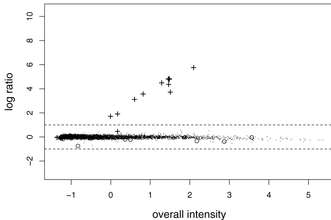
Figure 6. ANOVA-Normalized Log Ratio Estimates Without Background Subtraction for the HIV Data (---- two-fold change, y = \pm 1 ; \circ negative control; + positive control). Not subtracting the background shrinks the estimates toward the x -axis. One of the genes known to be differentially expressed shows a less than two-fold change, whereas it does not do so with background-subtracted data.
