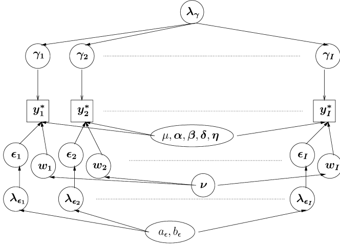
Figure 3. Directed Acyclic Graph of the General Model in (1).
