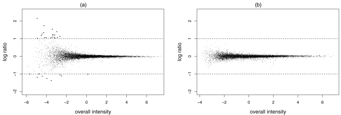
Figure 4. Log Ratio Estimates as a Function of the Overall Intensity (i.e., the average of the gene effects in each sample) on the Like-Like Data (first four replicates). (a) Like-like: least squares estimates (without shift); (b) like-like: posterior means. Using our method (b), 26 gene outliers were filtered out. The dashed lines show a two-fold change. The number of false positives for the normalized log ratios is 21, compared with only 0 for the posterior means, a 100% reduction.
